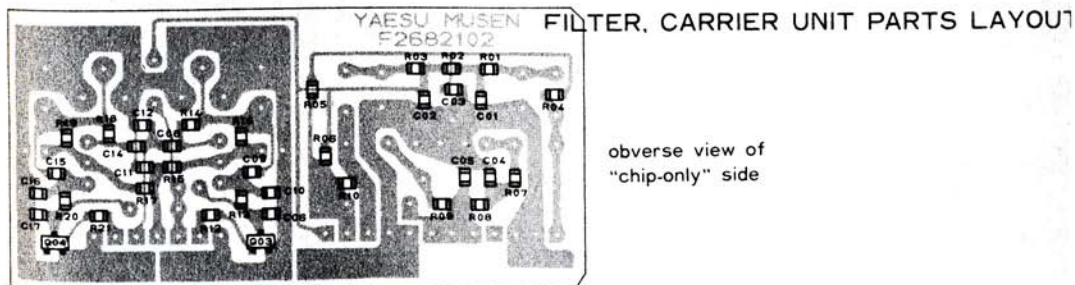
(reverse view of "component" side)
