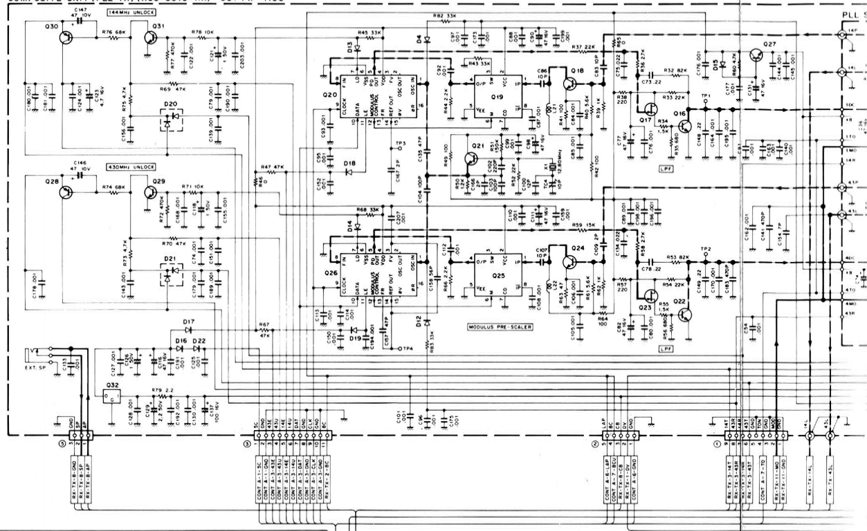
COMPOSITE UNIT (RX-TX) (X60-3000-XX) -00 TW-4100
