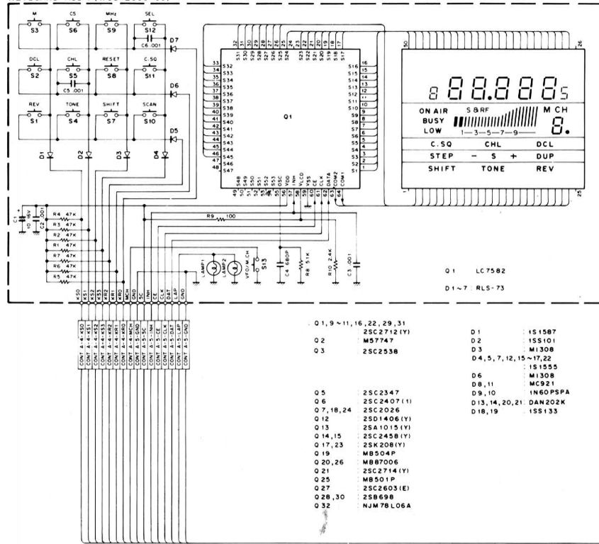
CONTROL UNIT (X53-3000-00) (A/4)
