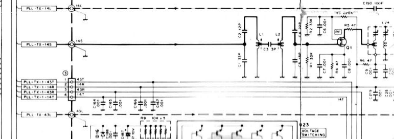
COMPOSITE UNIT (RX-TX) (X60-3000-XX) -00 TW-4100
